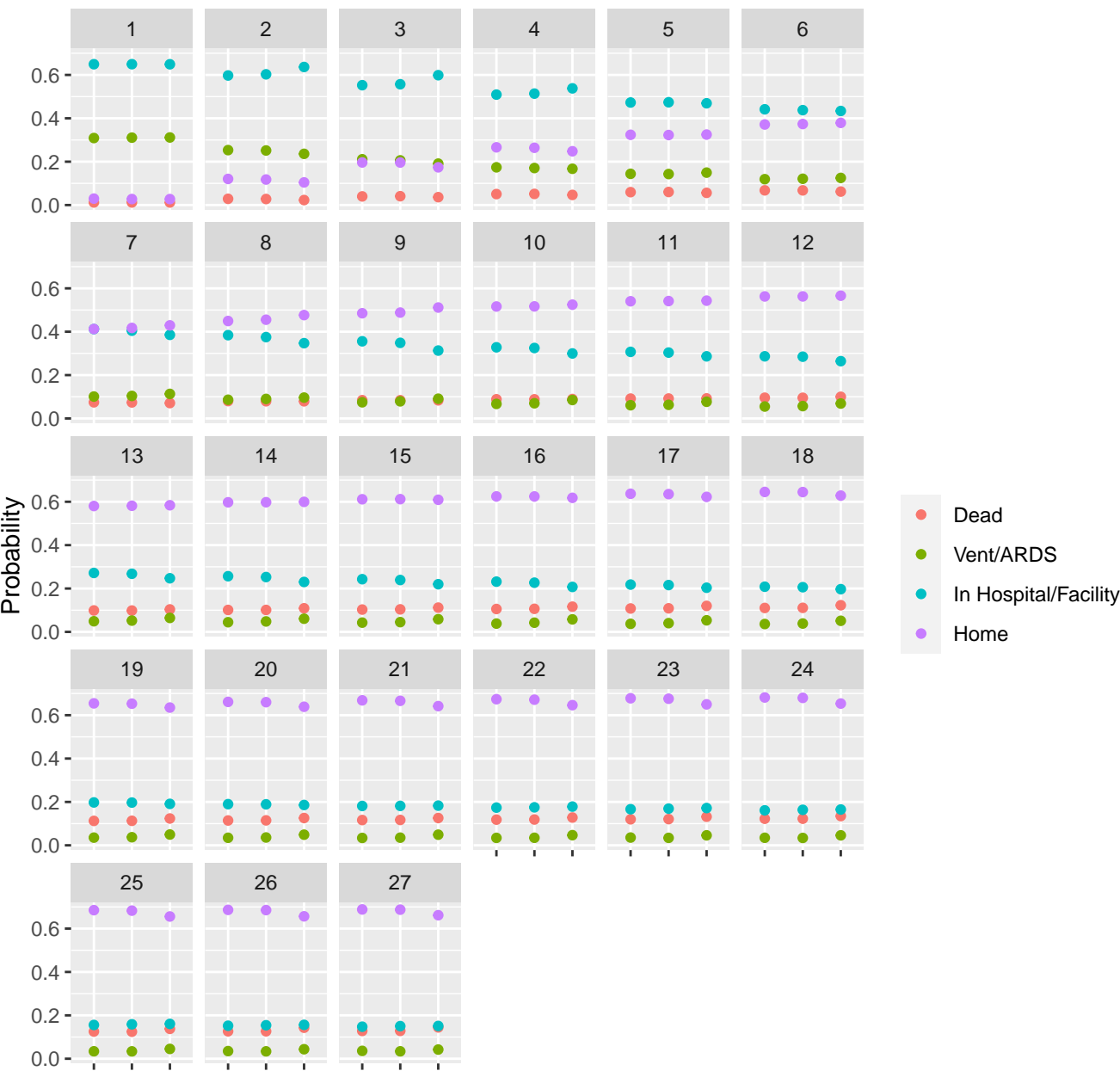
Simulated data, fitted model, and VIOLET 2 results (left to right)
